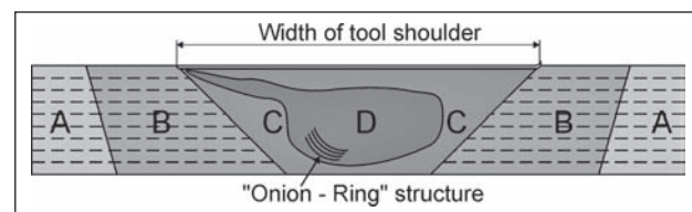
Figure 2 Various microstructural regions in the transverse cross section of friction stir welded material. A - unaffected material or parent metal, B - heat affected zone - HAZ, C - thermo-mechanically affected zone - TMAZ, D - "weld nugget" zone - NZ [1]
