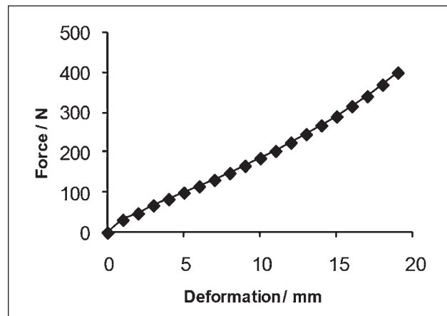
Figure 1 Stress-strain diagram of pneumatic-flexible element
