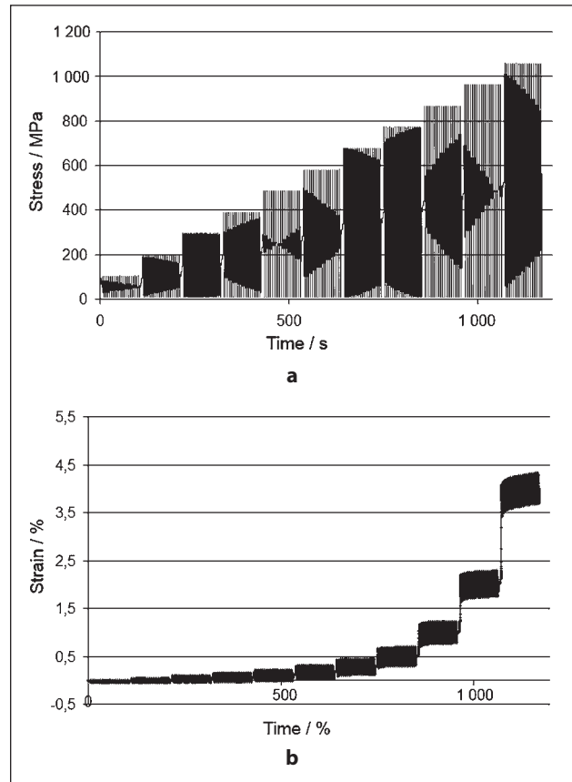
Figure 3 Examples of waveforms obtained by the MLCF test: a) the stress curve obtained for all „packages”, b) the strain curve obtained for all „packages”
