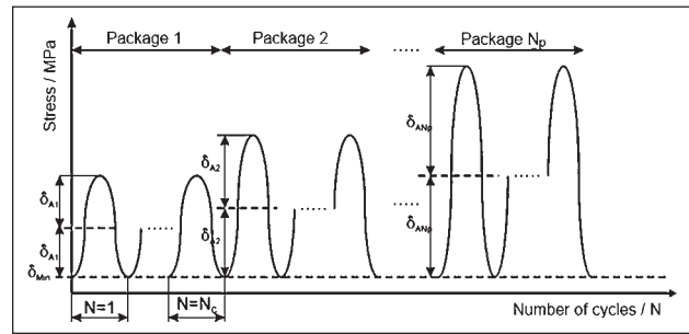
Figure 2 The run of a test programme
