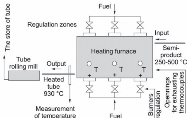
Figure 1 Heating furnace...
