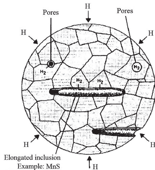
Figure 2 Positioning of molecular hydrogen in micro-pores [6]
