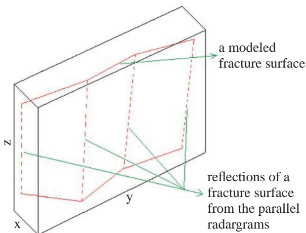
Figure 10: A model for an irregular 3D fracture surface resulting from tracing the belonging fracture reflections (dashed lines) in the radargrams. This fracture surface is the model of the fracture reflections presented in the garnet colour on the right hand side of Figure 9 . The black rectangle is a simulation of a partial body of the bench and it is used in this figure for better visualization of the fracture surface.
