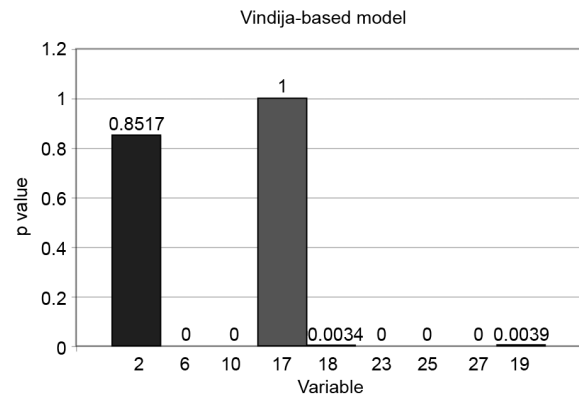
Fig. 7. Analysis of sample bias results: Scenario 3. P Values given in the plot are the proportion of 10,000 random, n = \text{Krapina } n samples with a mean greater than the observed Krapina mean. For each variable, the 10,000 samples are drawn from the upper half of a simulated population based upon Vindija's mean and standard deviation.
