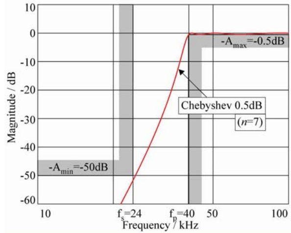
Fig. 12. The specifications and the Chebyshev HP filter transfer function magnitude
