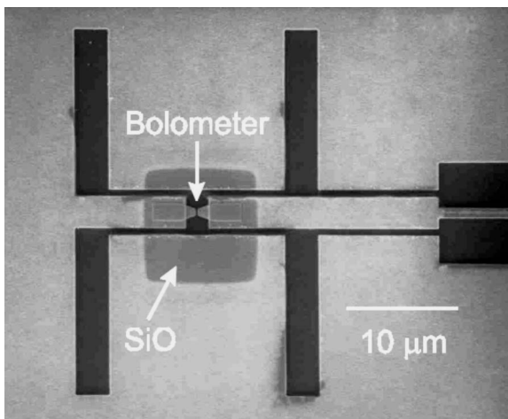
Fig. 1 SEM photo of an HEB mixer embedding circuit. The superconducting micro-bridge is located at the center and coupled to the twin-slot antenna via CPW lines
