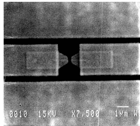
Fig. 2 SEM photo of a tapered bolometer-to-CPW transition. The gap length in this case is 0.2 \mu\text{m}
