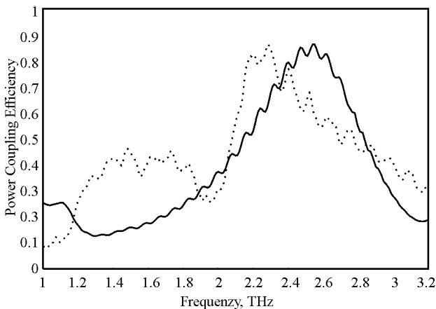
Fig. 4 Comparison between measured (dotted) and calculated (solid) power coupling efficiencies
