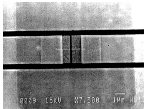
Fig. 3 SEM photo of a non tapered bolometer-to-CPW transition. The gap length here is just 0.1 \mu\text{m} .
