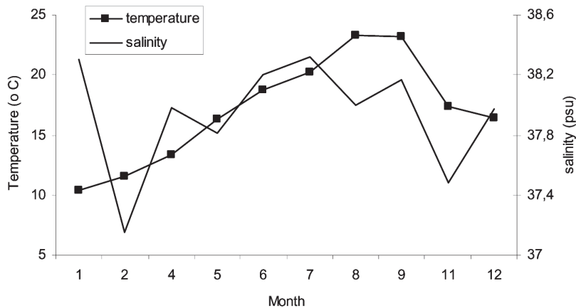
Fig. 3. Monthly temperature and salinity in the Kaštela Bay in 2002
