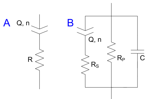
Fig. 3. Electrical equivalent circuits A and B
