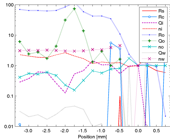
Fig. 13. Normalized equivalent circuit parameters depending on the file tip position - circuit F
