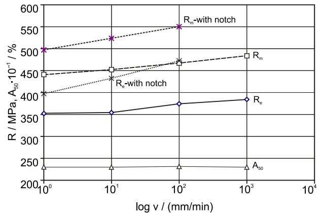
Figure 4. Influence of the loading rate on the mechanical properties of the tested sheet thick 1 mm Slika 4. Utjecaj brzine zatezanja na mehanička svojstva ispitivane trake debljine 1 mm
