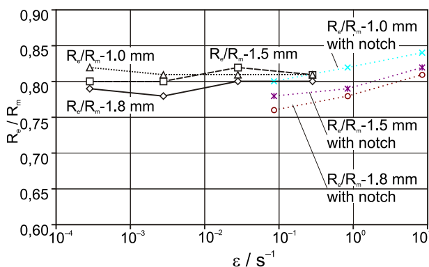
Figure 9. Influence of the strain rate \dot{\epsilon} on the R_e/R_m ratio of the tested sheets
