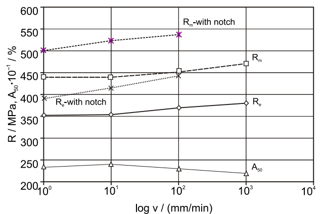
Figure 5. Influence of the loading rate on the mechanical properties of the tested sheet thick 1,5 mm Slika 5. Utjecaj brzine zatezanja na mehanička svojstva ispitivane trake debljine 1,5 mm
