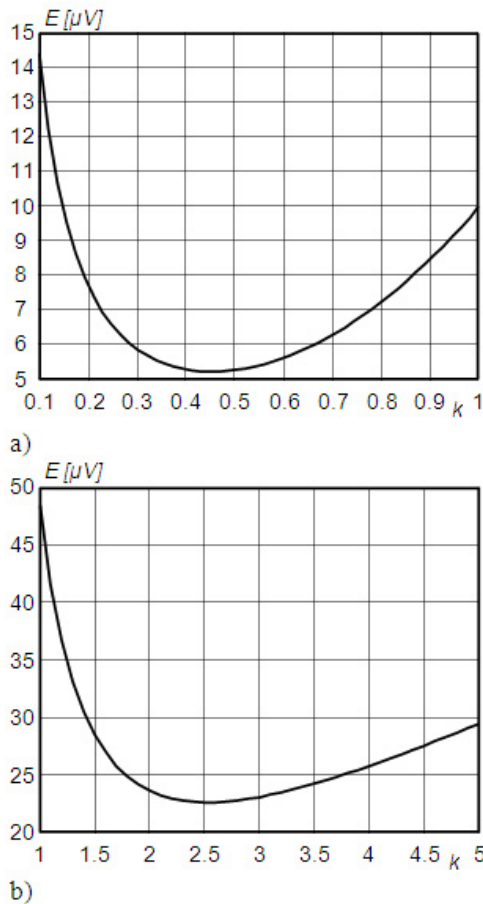
Fig. 8. RMS voltage as function of k ; a) LP, b) BP filter
