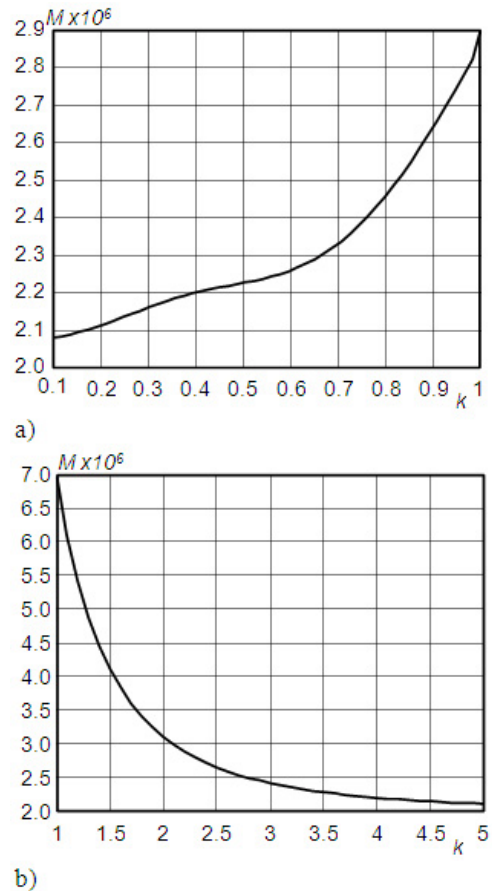
Fig. 9. Multi-parameter sensitivity measure as function of k ; a) LP, b) BP filter
