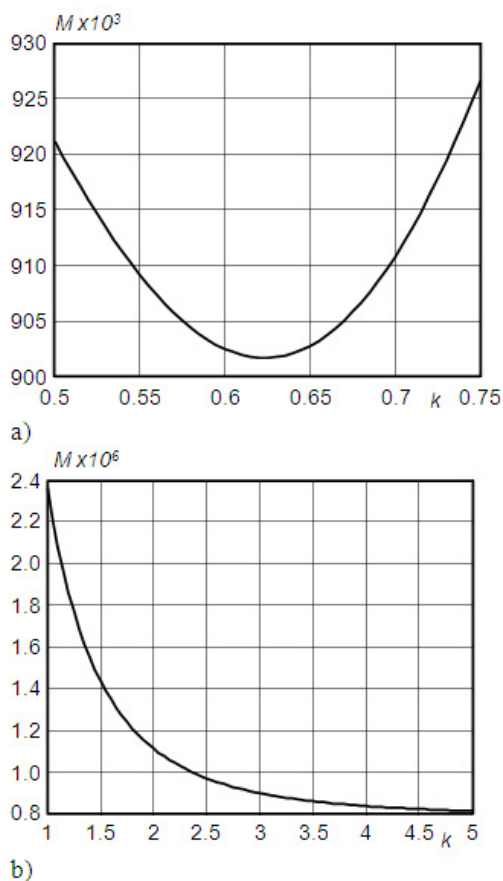
Fig. 4. Multi-parameter sensitivity measure as function of k ; a) LP, b) BP filter
