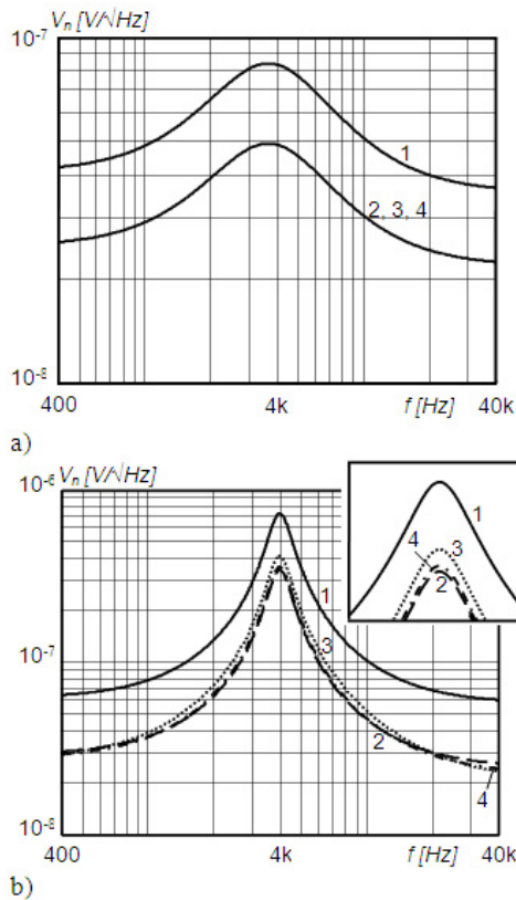
Fig. 5. Noise voltage spectral density for: 1. SD, 2. NO, 3. SO and 4. NSO of the 2 nd order; a) LP, b) BP filter
