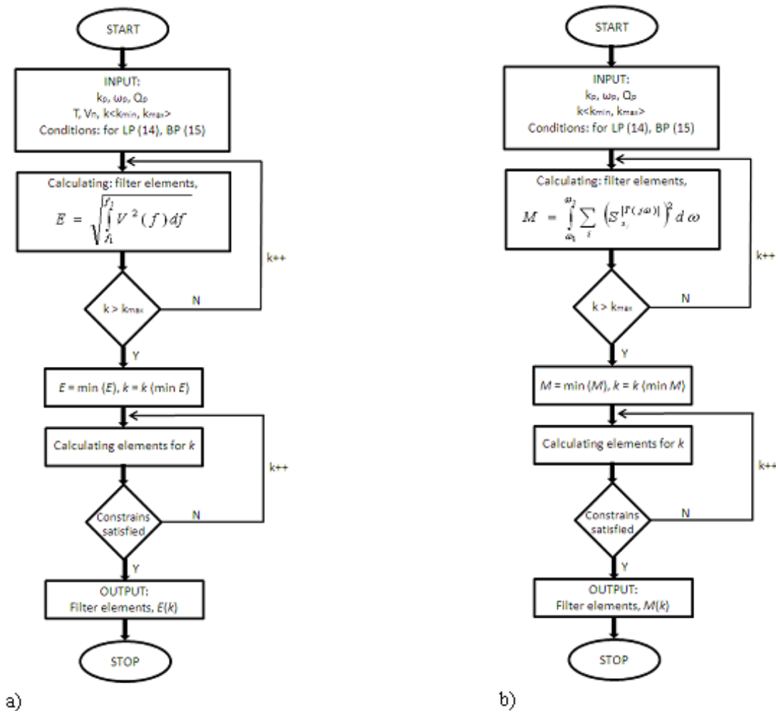
Fig. 2. Block-diagram for obtaining filters elements for; a) minimum noise, b) minimum sensitivity
