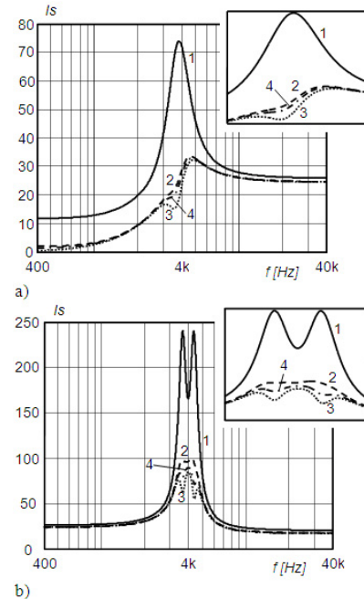
Fig. 13. Schoeffler sensitivity for: 1. SD, 2. NO, 3. SO and 4. NSO of the 4 th order; a) LP, b) BP filter
