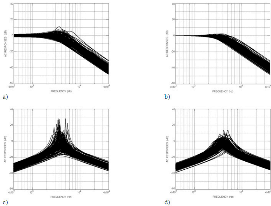
Fig. 16. Monte Carlo response plots of the 2 nd order; a) LP simple design, b) LP sensitivity optimized, c) BP simple design, d) BP sensitivity optimized
