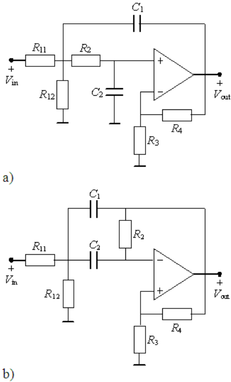
Fig. 1. The 2 nd order; a) LP, b) BP filter section
