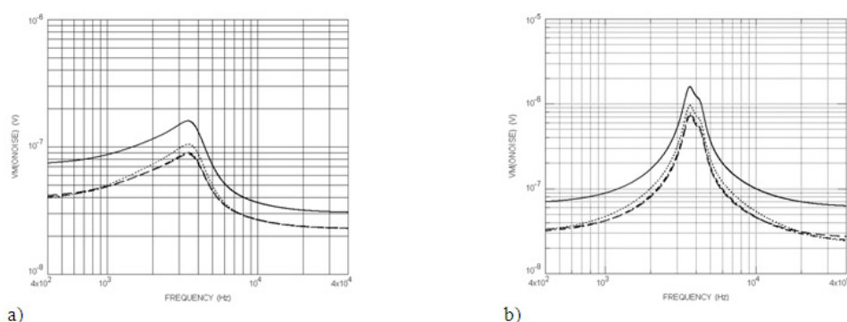
Fig. 15. Noise voltage spectral density using Spice of the 4 th order; a) LP, b) BP filter
