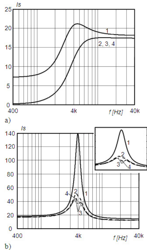
Fig. 6. Schoeffler sensitivity for: 1. SD, 2. NO, 3. SO and 4. NSO of the 2 nd order; a) LP, b) BP filter
