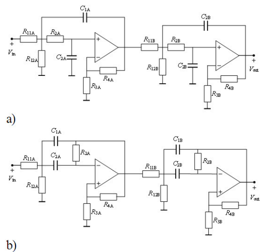
Fig. 7. The 4 th order; a) LP, b) BP filter
