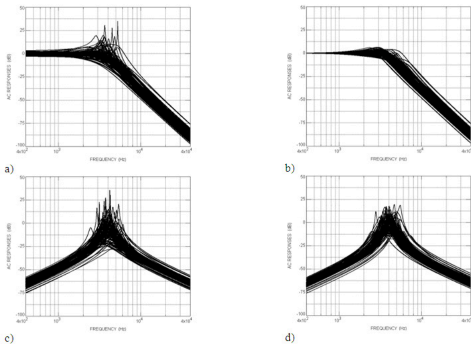
Fig. 17. Monte Carlo response plots of the 4 th order; a) LP simple design, b) LP sensitivity optimized, c) BP simple design, d) BP sensitivity optimized
