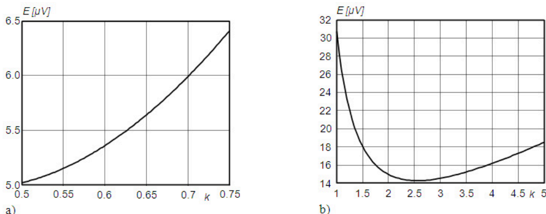
Fig. 3. RMS noise voltage as function of k ; a) LP, b) BP filter
