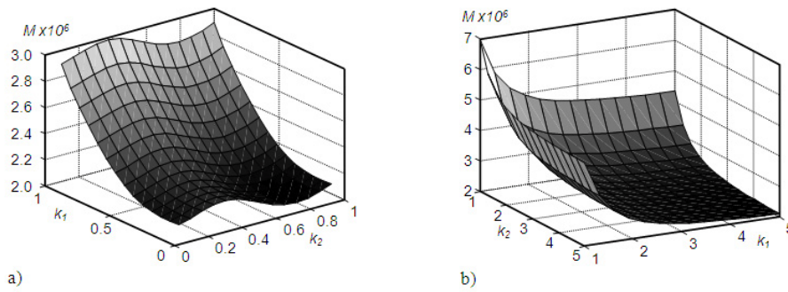
Fig. 11. Multi-parameter sensitivity measure as function of k_1 and k_2 ; a) LP, b) BP filter
