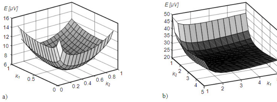
Fig. 10. RMS voltage as function of k_1 and k_2 ; a) LP, b) BP filter
