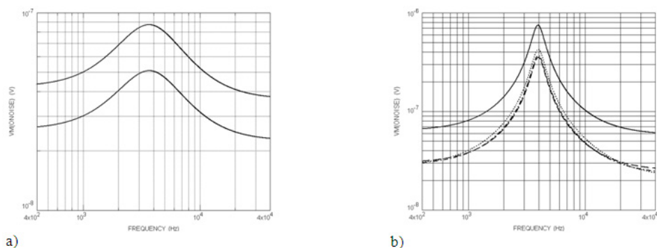
Fig. 14. Noise voltage spectral density using Spice of the 2 nd order; a) LP, b) BP filter
