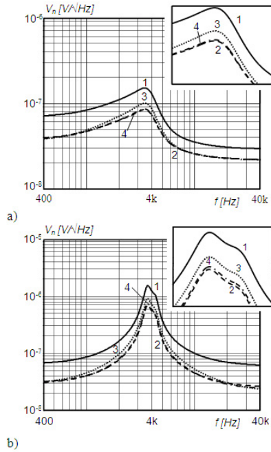
Fig. 12. Noise voltage spectral density for: 1. SD, 2. NO, 3. SO and 4. NSO of the 4 th order; a) LP, b) BP filter
