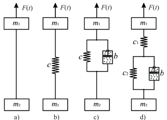
Figure 6 Dynamic model of a supporting element, inelastic element (a), Hook's model (b), Calvin's model (c) and a standard model (d)
