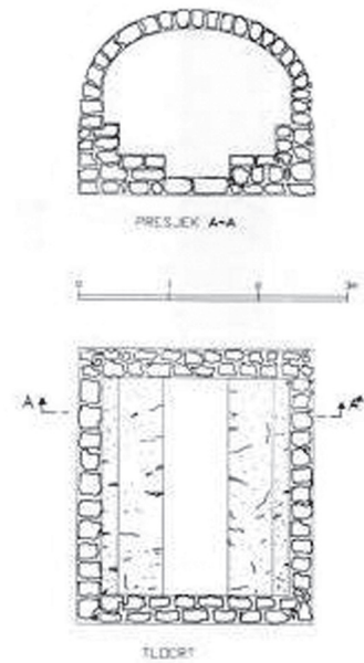
Sl. 6. Grobnica na svod u Previšu, tloris i presjek. Fig. 6. Vaulted tomb in Previš, layout and cross-section.
