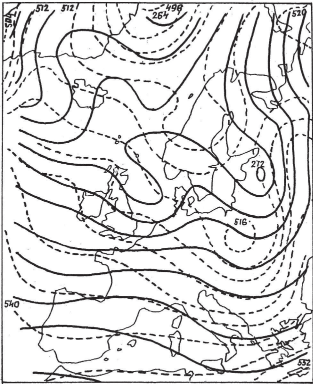
SL.3.3.2.2.(iii) AT 700 RT 500 1000 29.1.1952. 03h
