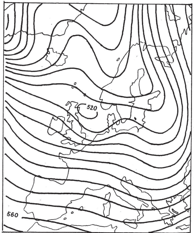
SL.3.3.2.2.(ii). RT 500 29.I.1952. 03h
