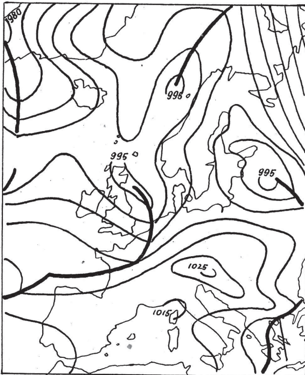
SL.3.3.2.2.(i) 29.I.1952. 00h
