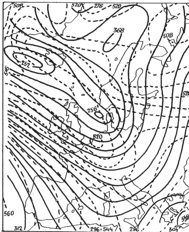
SL.3.3.2.2(xii). RT 700 RT 500 RT 1000 1.11.1952. 03h
