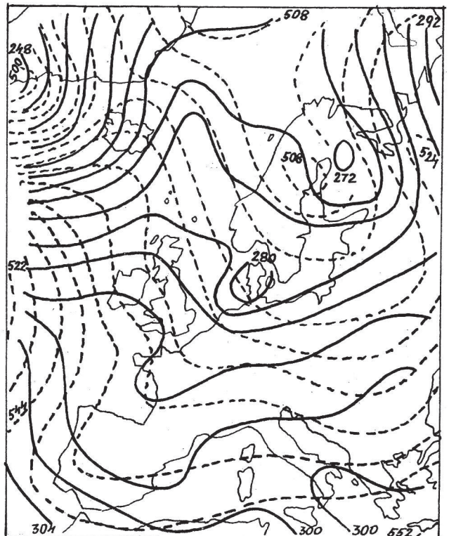
SL.3.3.2.2.(vi.) AT 700 RT 500 1000 30.1.1952 03h
