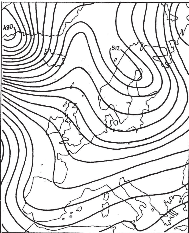
SL.3.3.2.2.(v). AT 500 30.1.1952. 03h
