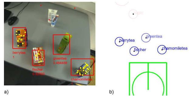
Fig. 5. Object Recognition: a) the camera image with rectangular object regions that are computed from LRF object detections. The image also shows extracted SURF features (yellow dots) and recognized object class. b) recognized objects are tracked in egocentric coordinates by a Kalman filter.
