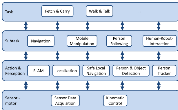
Fig. 4. Overview over the control modules within Dynamaid's behavior architecture.
