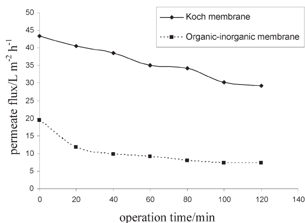
Fig. 3 – Comparison of G. robertianum extract flux values at different NF membranes vs. time
