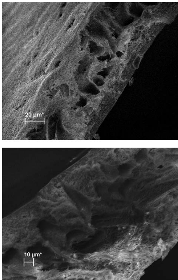
Fig. 2 – Morphology of nanofiltration organic-inorganic membranes from SEM
