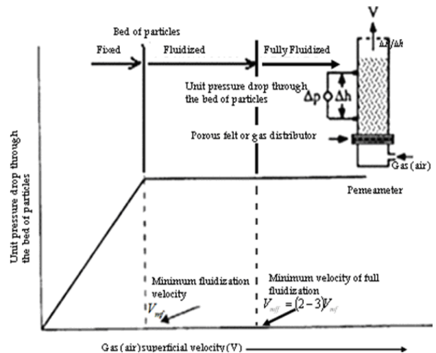
Figure 5. Pressure drop through a bed of uniformly particles versus superficial air velocity – source: (Mills, 1990) 12 .
