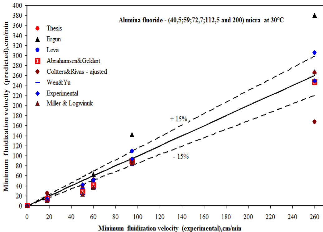
Figure 13. Comparison of experimental values of V_{mf} with predicted values
