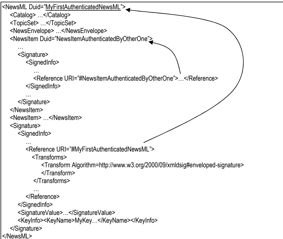
Figure 5: Example of an authenticated NewsML element
