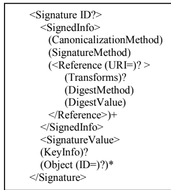
Figure 2: XMLDSig Signature structure
