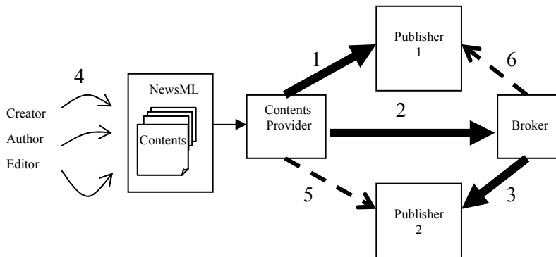
Figure 3: NewsML Scenario
