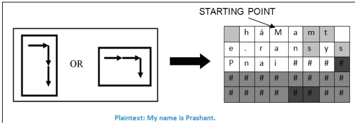
Figure 2. Knight Movement Pattern and its implementation in the golden rectangle
