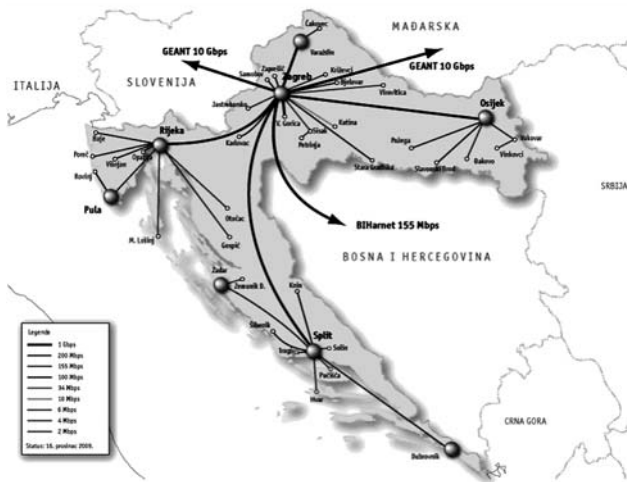
Figure 7 CARNet network
