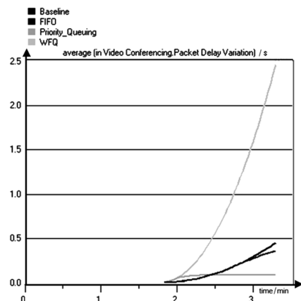
Figure 15 Packet delay variation, TSF = 0,5
