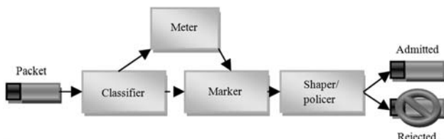
Figure 2 Packet classification procedure
