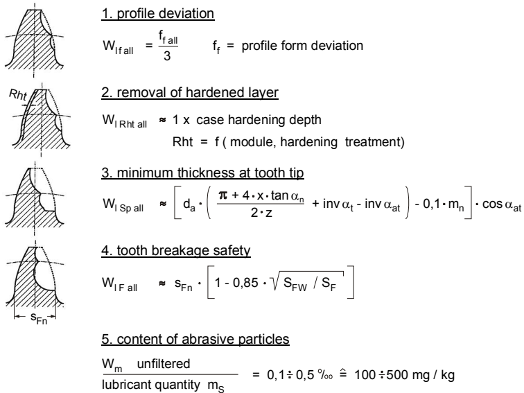
Figure 7: Allowable wear amount acc. to [7]
