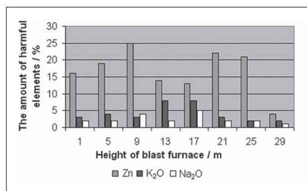
Figure 1 Content of zinc and alkaline carbonates in the lining
