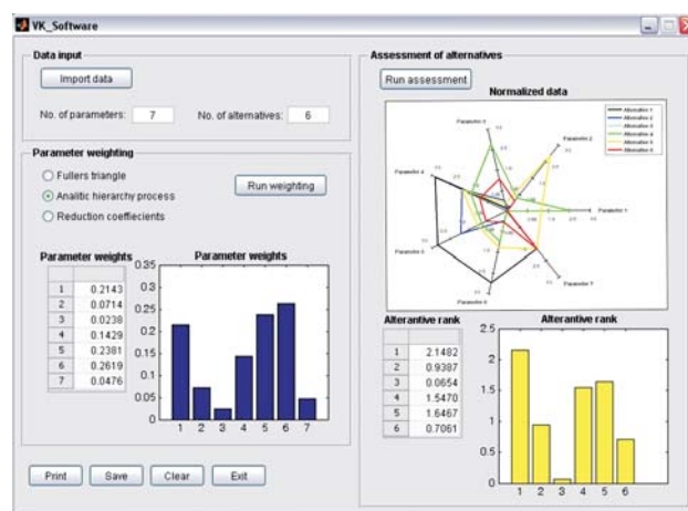
Figure 3 VK Software main panel [1]
