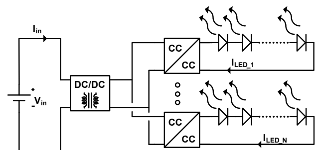
Fig. 10. DC-DC two-stage active solution with galvanic isolation
