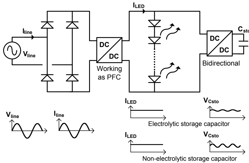
Fig. 17. Special two-stage topology with bidirectional auxiliary converter
