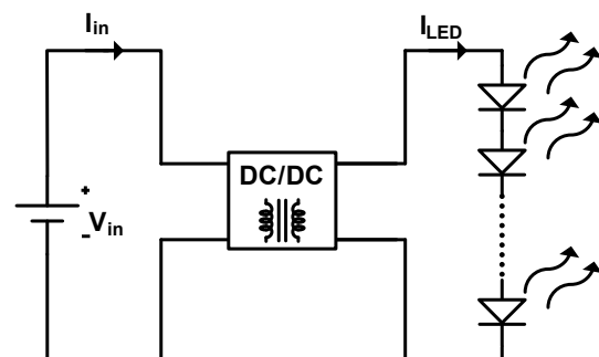
Fig. 8. DC-DC one-stage active topology with galvanic isolation
