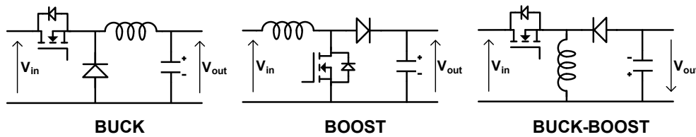
Fig. 6. Most common non-isolated DC-DC topologies. The buck and the buck-boost topologies can be modified for HB-LEDs applications so that their MOSFET is referred to ground.
