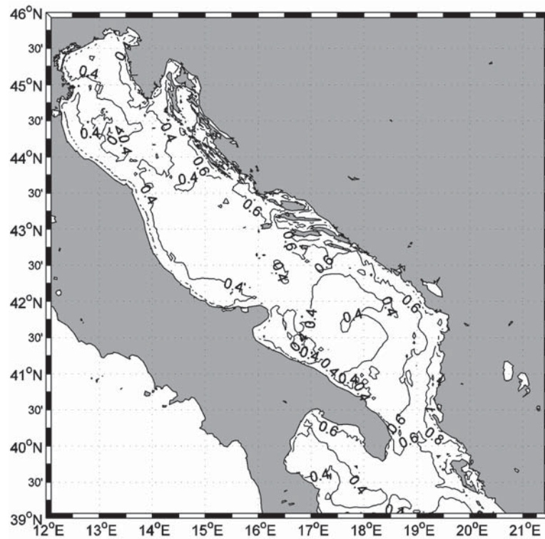
Fig. 12. Horizontal map of the time averaged (from 1 April to 31 December 2003) RMS error between hindcasted and forecasted SST. Units are °C
