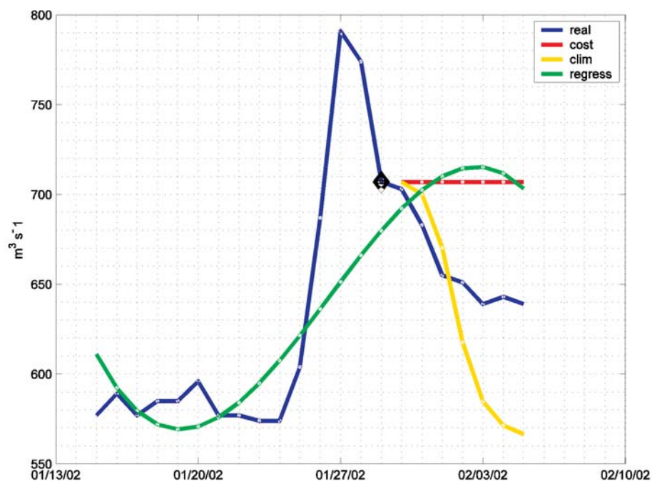
Fig. 4. Example of Po runoff forecasts for the week from 29 January 2002 to 5 February 2002. The diamond indicates the last available Po data. In blue the observed runoff is reported. Green, red and yellow indicate the results of the different forecast methods tested
