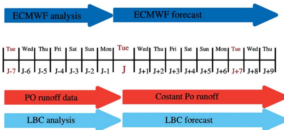
Fig. 3. Time line of hindcast-forecast procedure. The arrows indicate the external data collected and used for the model simulations. 'LBC' indicates the large scale model data used for Lateral Open Boundary conditions. The analysis data span the period starting from noon of the previous Tuesday (J-7) to noon of the current Tuesday (J). The forecast data span the period from 6.00 p.m. of the current Tuesday (J) to Thursday of the next week
