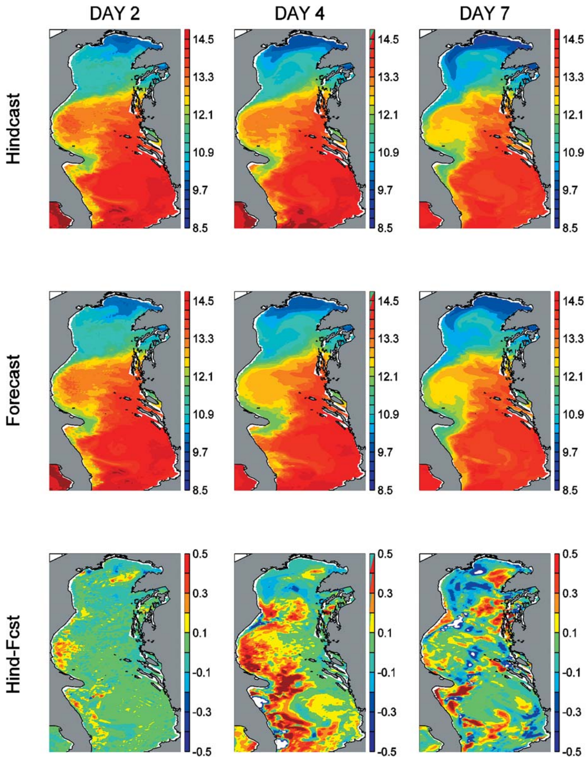
Fig. 10. Horizontal maps of near surface (2 m depth) hindcasted and forecasted temperature and their differences. The two simulations (hindcast and forecast) started on 1 April 2003. The second, fourth and seventh days of the simulations are shown. Units are °C
