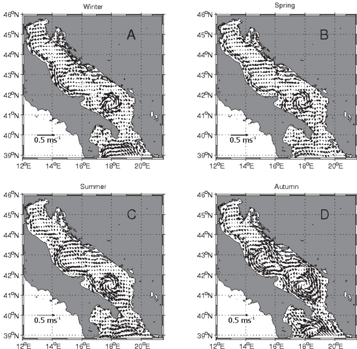
Fig. 6. Seasonally averaged (for year 2003) near surface (2 m depth) velocity field. Winter from January to April (panel A); spring from May to June (B); summer from July to October (C); autumn from November to December (D). The seasons definition was first proposed by ARTEGIANI et al. (1997 a,b)
