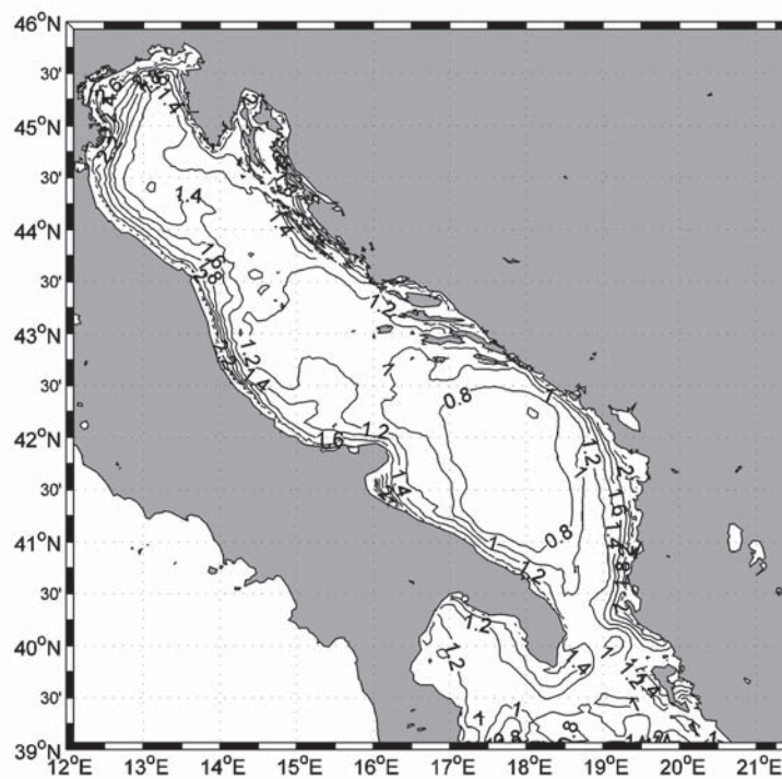
Fig. 8. Spatial distribution of the annually averaged (from 1 January to 31 December 2003) hindcast RMS error computed using the (remotely) observed and hindcasted SST. Units are °C
