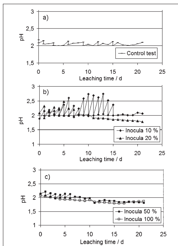
Figure 1 Variation of pH during leaching process with variable quantities of At. Ferrooxidans : a) control test (0 %); b) 10 % and 20 %; c) 50 % and 100 % of inocula
