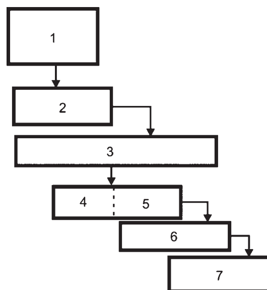
Figure 2 Deposit deoiling installation by Eko-Fortuna; 1 - dosing tank, 2 - conveyor, 3 - heating chamber, 4 - water condenser, 5 - oil condenser, 6 - cooler, 7 - storage centre [12]
