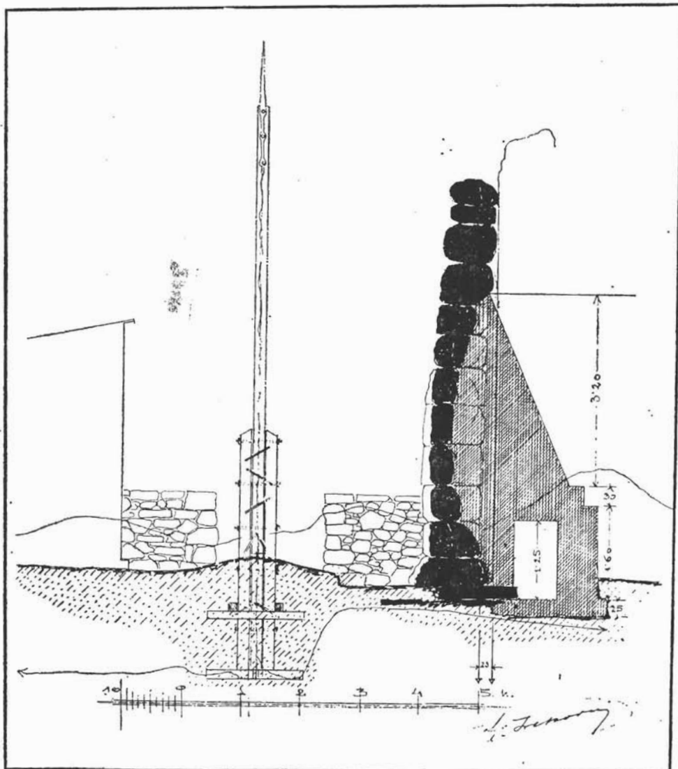
Sl. 5. Č. Iveković, projekt za osiguranje lukova u Burnumu. Poprečni presjek u kojemu se sasvim lijevo vidi rub barake podignute prilikom arheoloških istraživanja. U sredini je gromobranski stup za zaštitu lukova od udara groma i desno trošni pilastar lukova otraga poduprt betonskom masom. — Č. Iveković, the proposed consolidation of the arches in Burnum. Transverse section — on the far left the edge of the hut erected during the archaeological investigations is visible. In the middle is the lightning conductor for the protection of the arches and on the right a crumbling arch pilaster supported by concrete
