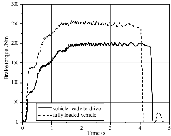
Figure 9 Influence of the vehicle's weight on the brake torque (initial speed 80 km/h)
