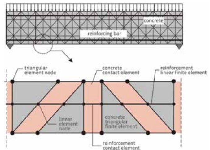
Figure 5. Discretization of RC structure
