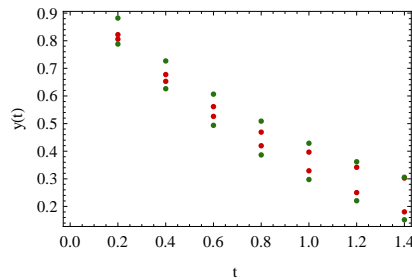
Figure 2: The results obtained for Example 1, by the proposed method (red dots) and AWA method (green dots)
