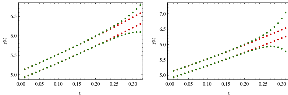
Figure 5: The results obtained for Example 3 by the proposed method (left, green dots) and AWA method (right, green dots) and the exact bounds (red dots)
