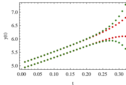
Figure 6: The results obtained for Example 3, by the proposed method (red dots) and AWA method (green dots)
