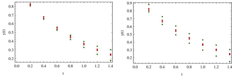
Figure 1: The results obtained for Example 1 by the proposed method (left, green), AWA method (right, green) and exact bounds (red)
