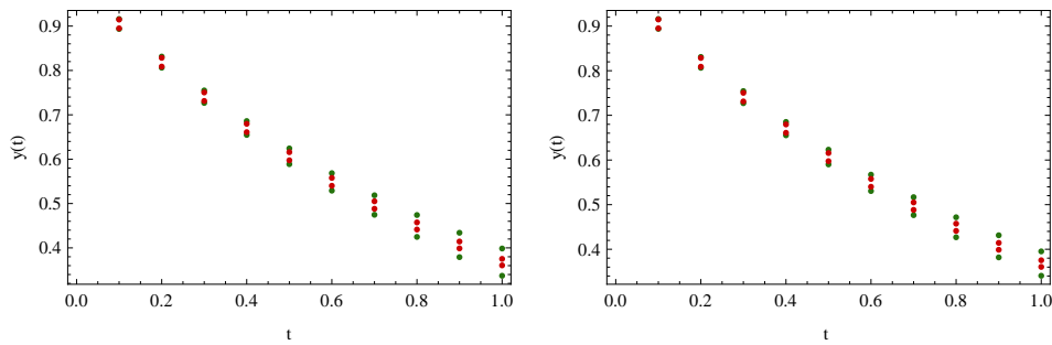
Figure 3: The results obtained for Example 2 by the proposed method (left, green), AWA method (right, green) and exact bounds (red)
