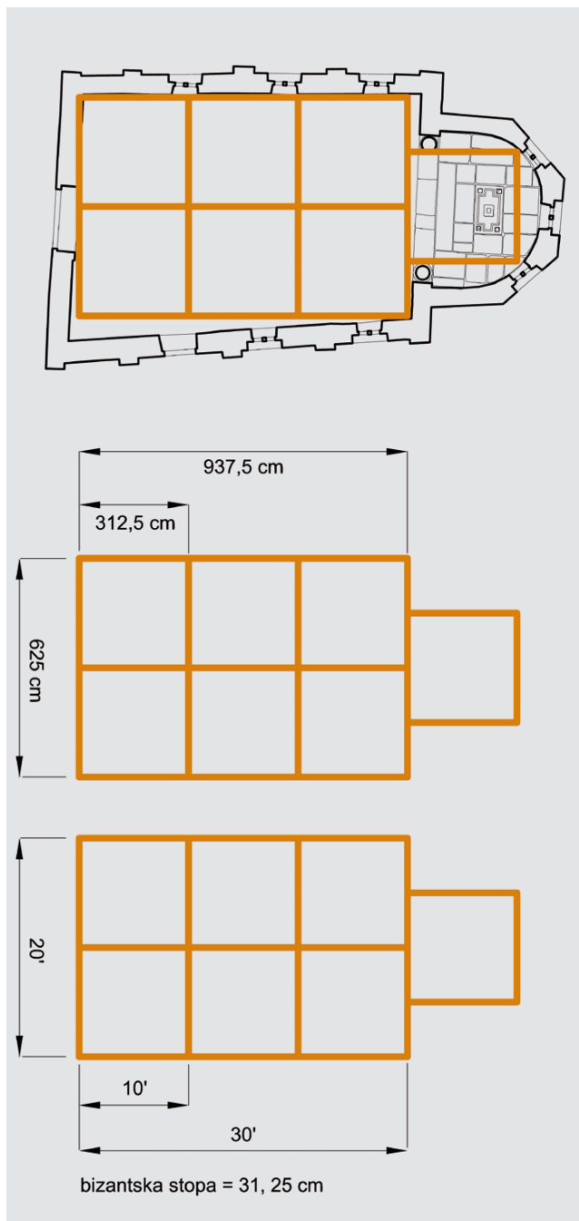
13. Prikaz razmjera tlocrta Ground plan and modular grid of St Nicholas'
