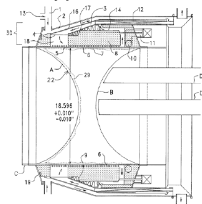
Figure 6. Sandia receiver [32].
