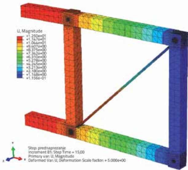
Figure 12. Truss girder displacements after prestressing
