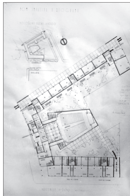
SL. 5. INVALIDSKI DOM U BEOGRADU, 1935. GODINE FIG 5 INVALIDS' CENTRE IN BELGRADE, 1935
