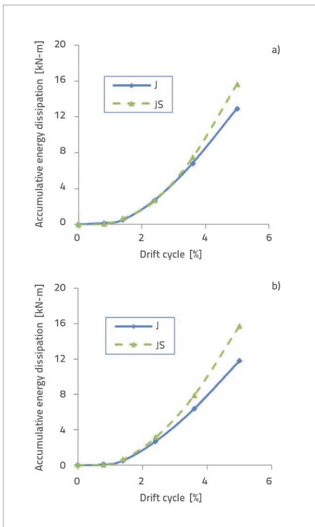
Figure 24. Accumulative energy dissipation capacity; a) Experimental; b) Analytical
