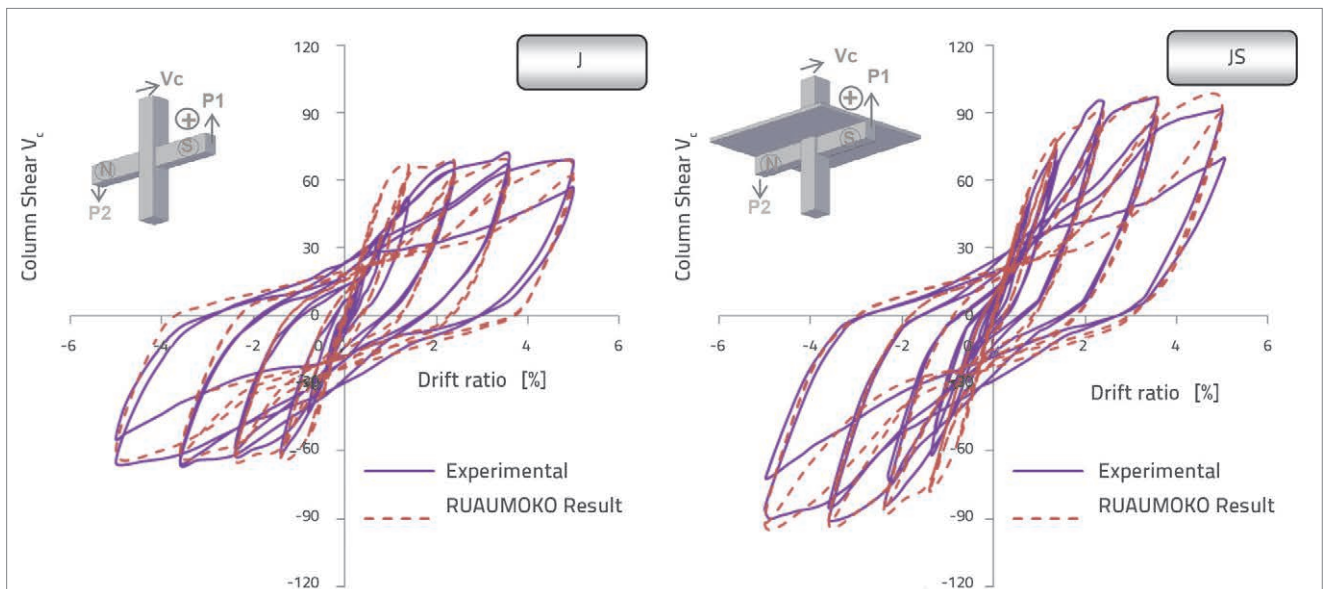
Figure 23. Simulation of hysteresis loops of column shear vs drift ratio
