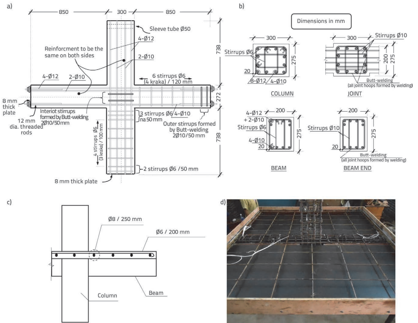
Figure 3. Reinforcement details of the specimens: a) Longitudinal reinforcement details (specimens J, JS); b) Section details (specimens J, JS); c) Section in the slab (specimen JS); d) Reinforcing view (specimen JS)
