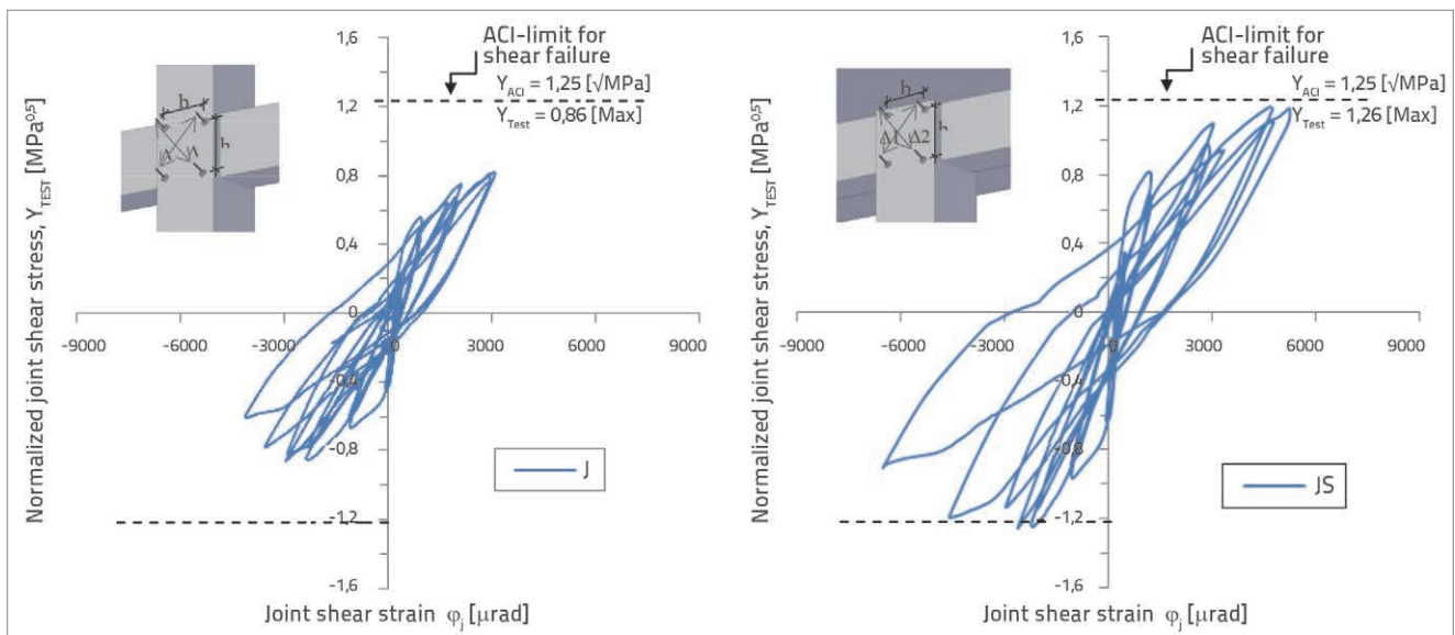
Figure 14. Normalized joint shear stress vs joint shear strain for the joints J and JS
