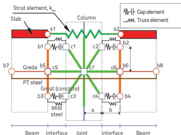
Figure 16. Development of the joint model
