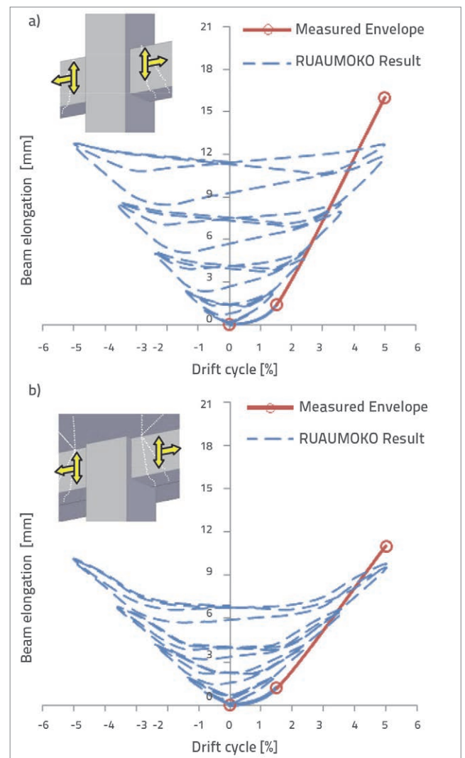
Figure 25. Beam elongation/relaxation vs drift ratio: a) Specimen J; b) Specimen JS
