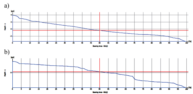
Figure 4 Load capacity curves a) after turning b) after FDM technology
