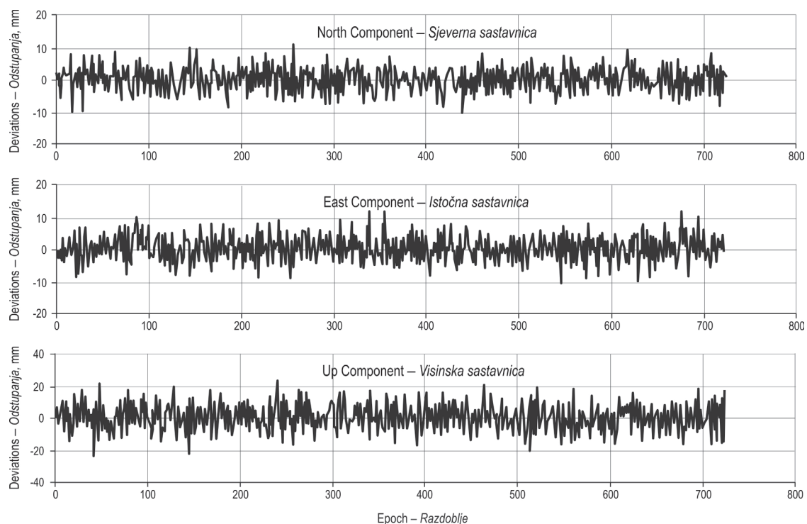
Fig. 12 Deviations of the components from averages for the \sigma\text{-}\Delta modeling
