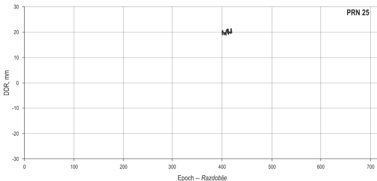
Fig. 6 Double difference residuals of PRN 25 for the baseline T_1-T_2
