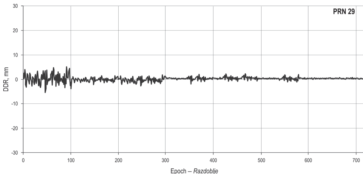
Fig. 5 Double difference residuals of PRN 29 for the baseline T_1-T_2
