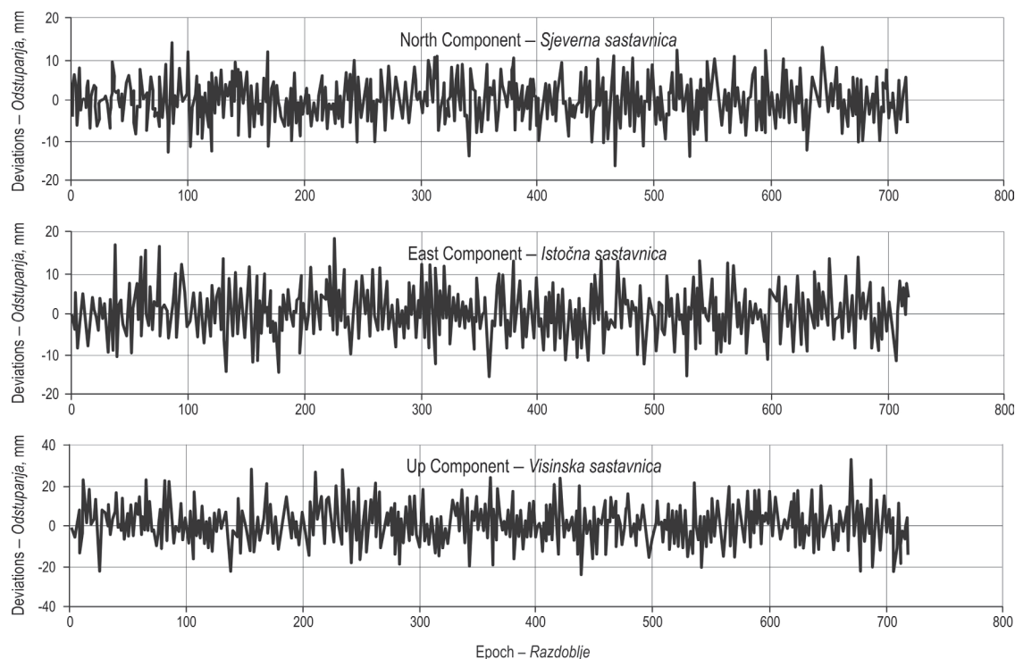
Fig. 13 Deviations of the components from averages for the \sin^2h/\text{SNR} modeling
