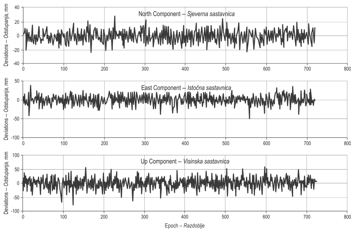
Fig. 11 Deviations of the components from averages for the equal variance modeling
