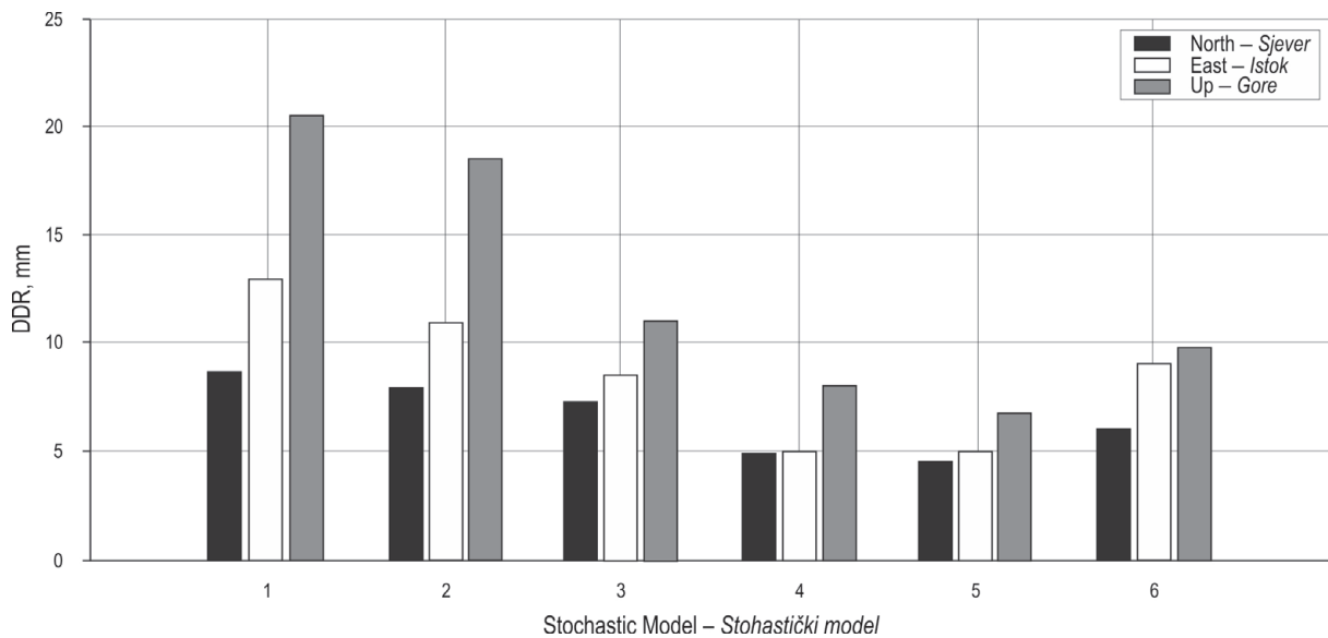
Fig. 10 Standard deviations from epoch by epoch processing of baseline T_1-T_2
