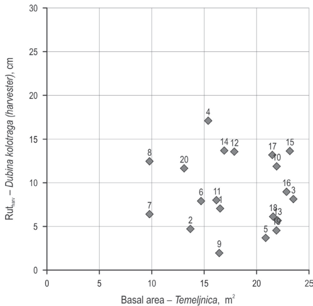
Fig. 4 Covariation between rut depth of harvester and basal area Slika 4. Ovisnost dubine kolotruga harvesteri i temeljnica
