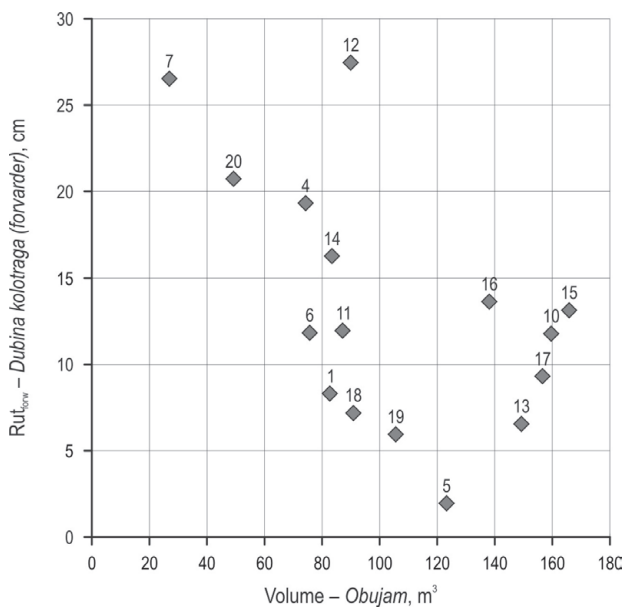
Fig. 6 Covariation between rut depth of forwarder and volume Slika 6. Ovisnost dubine kolotruga forvardera i obujma stabala
