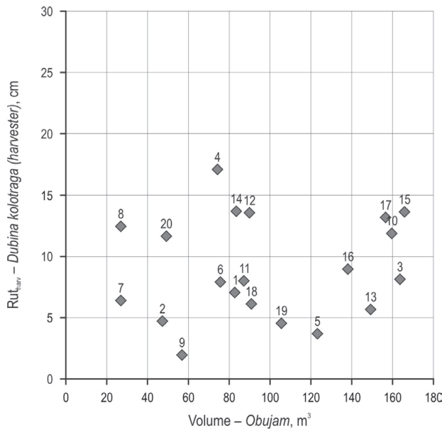
Fig. 3 Covariation between rut depth of harvester and volume Slika 3. Ovisnost dubine kolotruga harvesteri i obujma stabala
