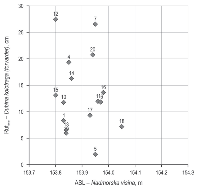
Fig. 8 Covariation between rut depth of forwarder and ASL Slika 8. Ovisnost dubine kolotruga forvardera i nadmorske visine
