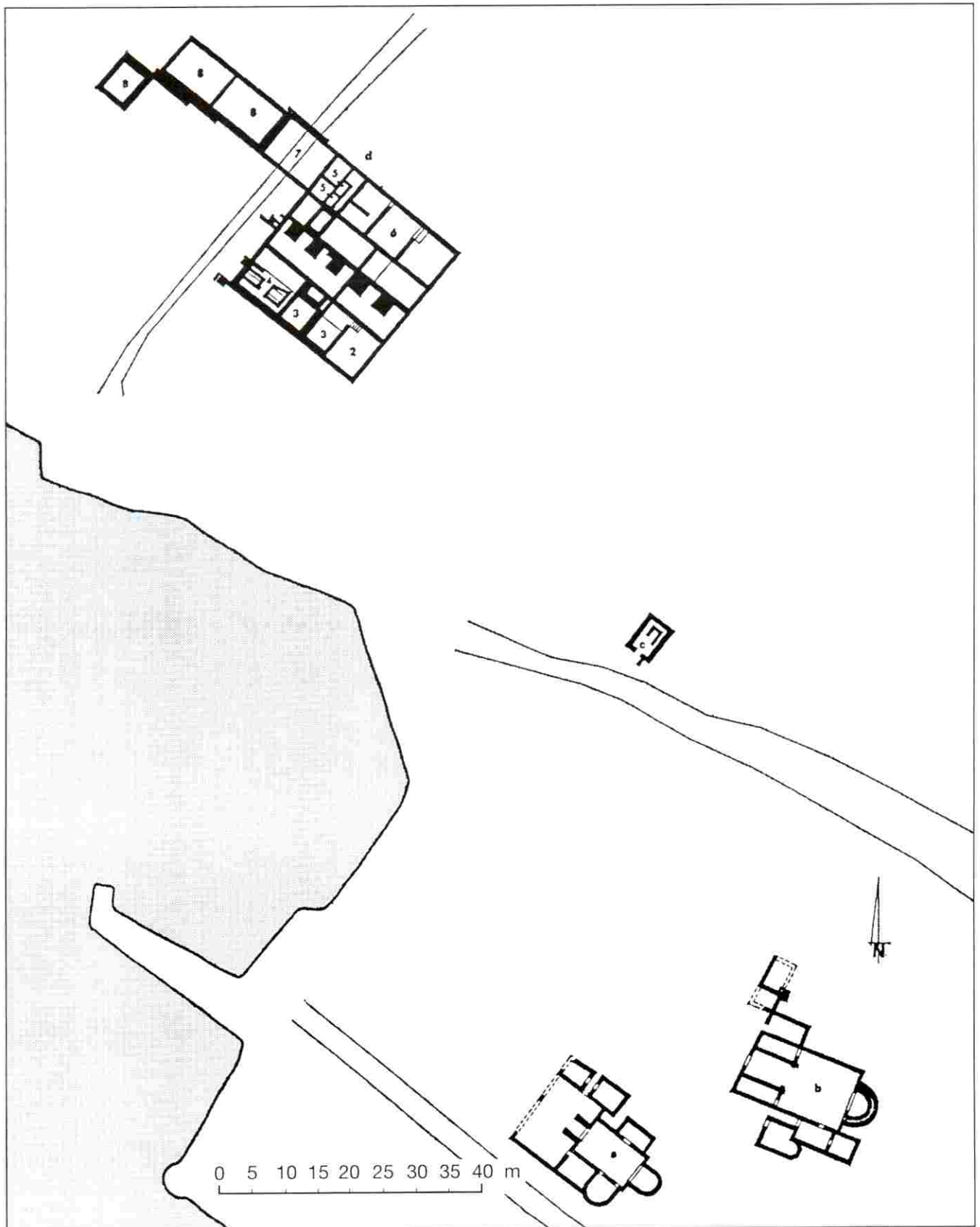
Fig. 8. Villa in Mulinie on the island of Ugljan (ground plan according to Suteu)
