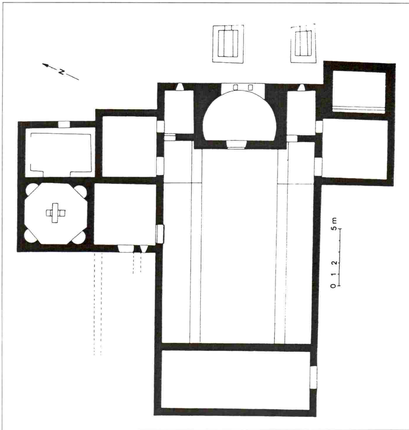
Fig. 11. Ground plan of the basilica in Povlja on the island of Brač (according to OSTOJČIĆ)
