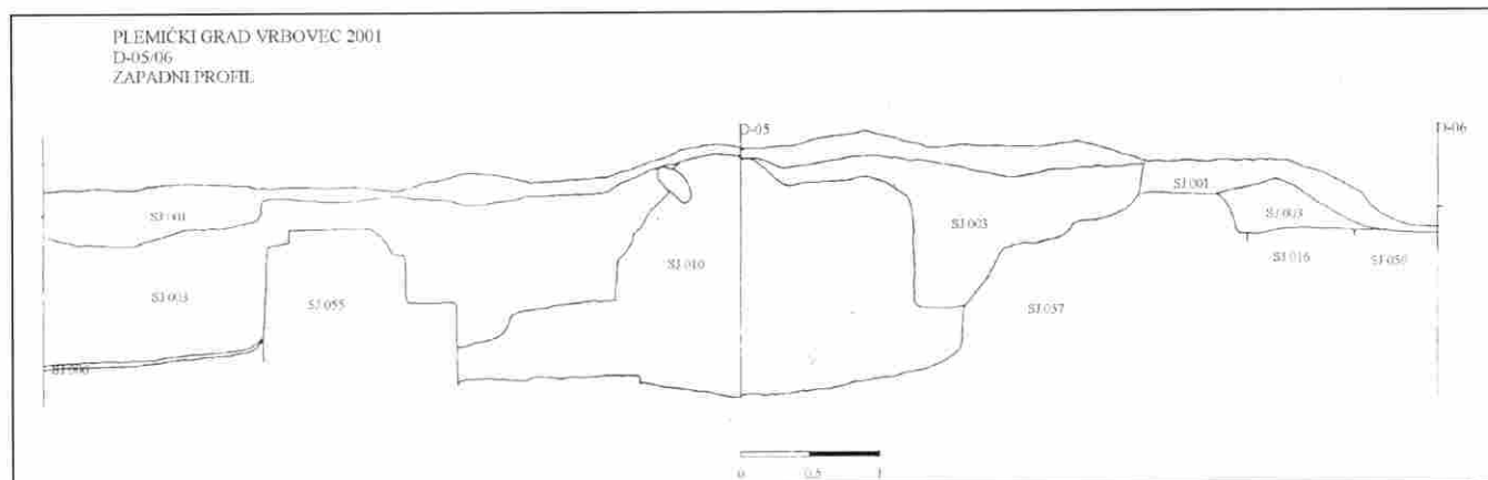
Fig. 19. Western profile of the north-eastern hall - stratigraphy
