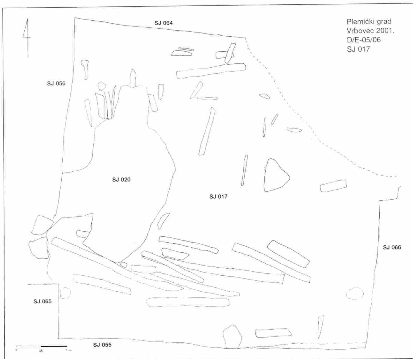
Fig. 13. Northeastern hall: ground-plan of the first implosion phase SU 017 (burned surface and burned, imploded roof-beams) and the remains of the construction of the tiled stove SU 020
