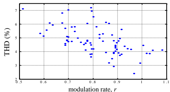
Slika 7. THD versus r for all switching angles
