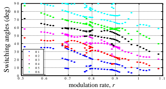
Slika 6. All switching angles versus r for a 13-level USAMI
