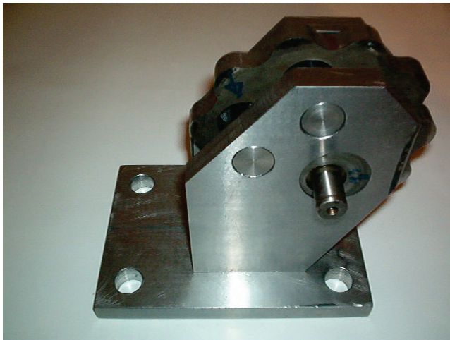
Figure 7 Physical model of the tool for investigation of the stress state of the cycloid disc
