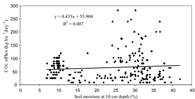
Fig. 6. Correlation between CO 2 efflux and soil moisture at 10 cm depth.
