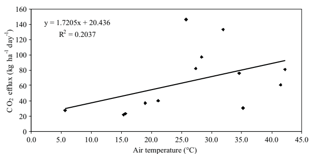
Fig. 8. Correlation between CO 2 efflux and air temperature.
