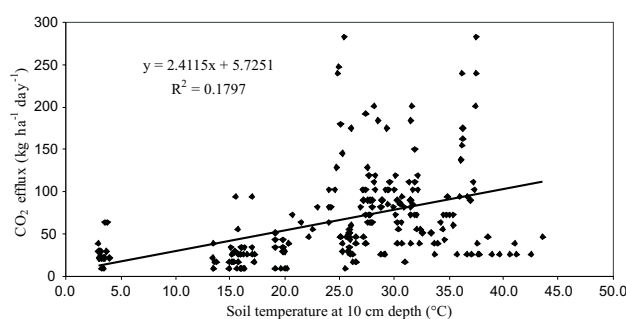
Fig. 7. Correlation between CO 2 efflux and soil temperature at 10 cm depth.
