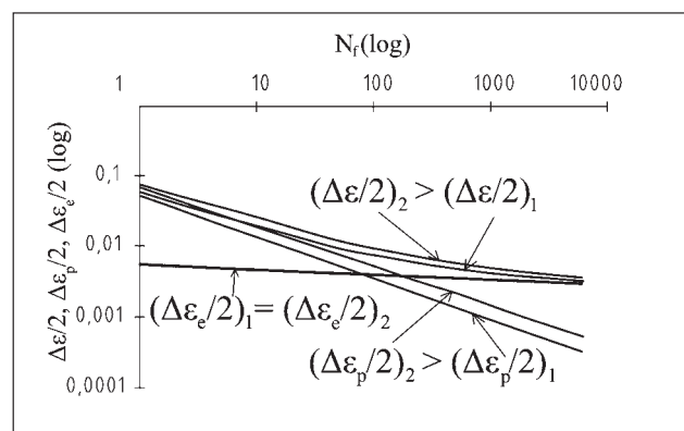
Figure 4 Strain-life curves for both versions
