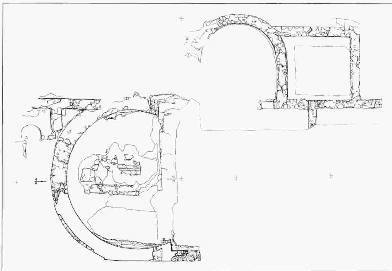
Fig. 11 Remnants of the building situated west of Palače, after the excavations lead by the Institute of Monuments Conservation - Dubrovnik.
