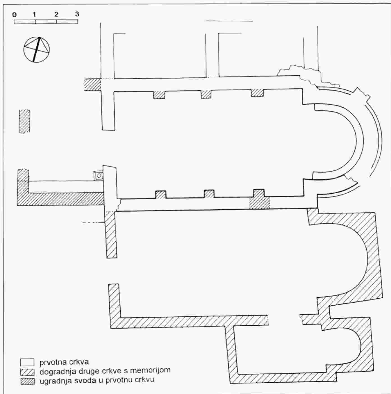
Fig. 18 The ground-plan of the church south-east of the palace - phases of the design
