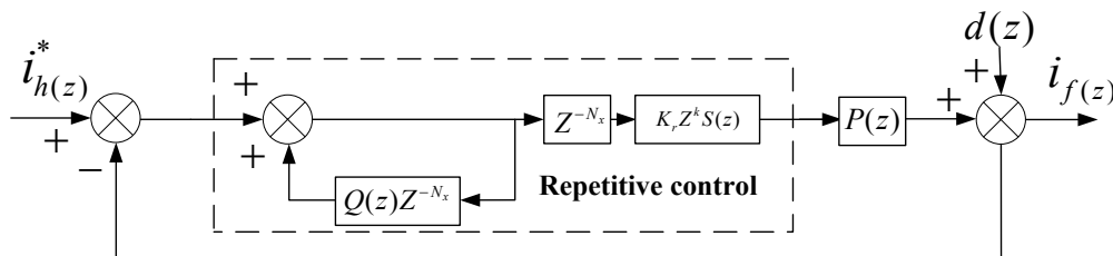
Figure 3 Conventional repetitive controller
