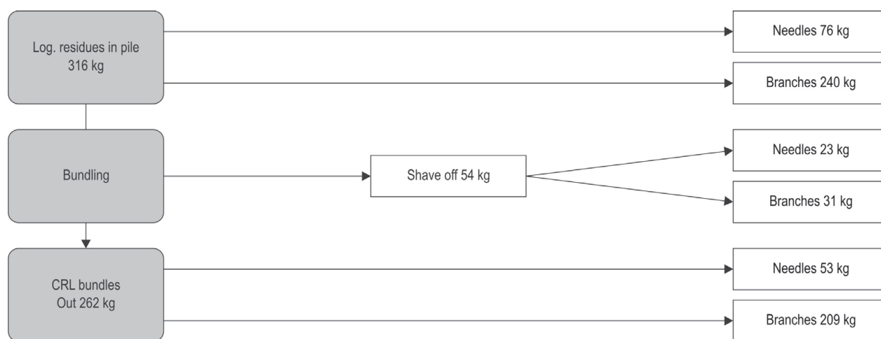
Fig. 6 Composition of material flow (kg DM) when producing one bundle including the peeled off material (Smland material)
