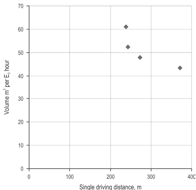
Fig. 7 Productivity when forwarding CRLs in terms of transported volume for a single driving distance
